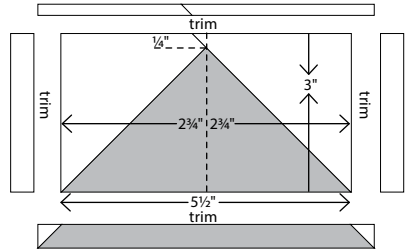
Roof 3" x 5 \frac{1}{2} " unfinished
